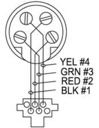
WIRE CONNECTIONS REAR VIEW (TYP)
