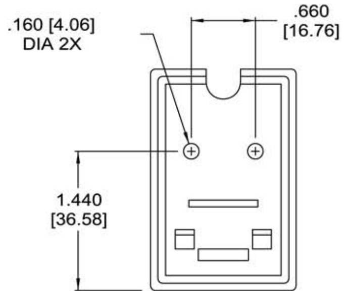
MOUNTING INFO
