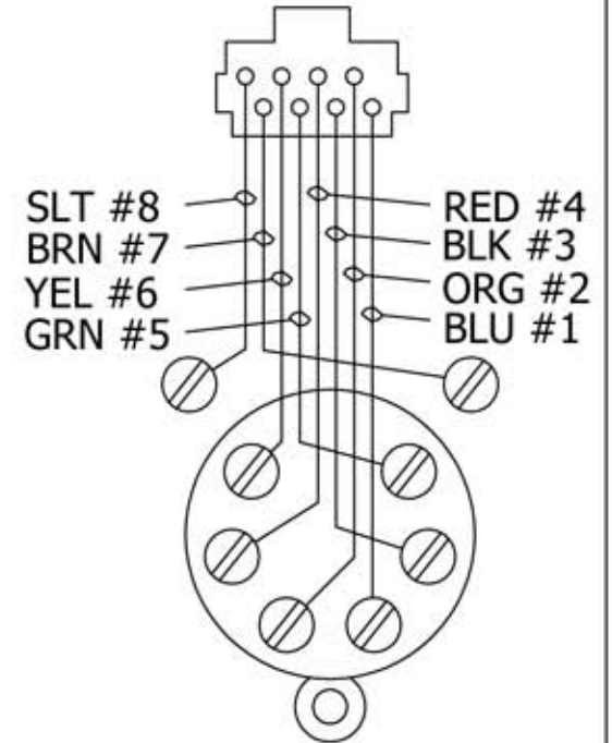
WIRE CONNECTIONS REAR VIEW (TYP)
