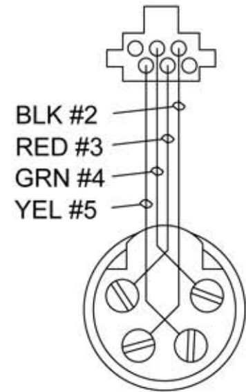
WIRE CONNECTIONS REAR VIEW
