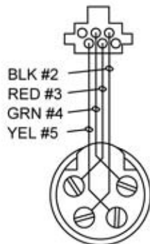
WIRE CONNECTIONS REAR VIEW
