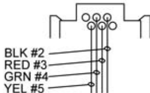
WIRING VIEW
