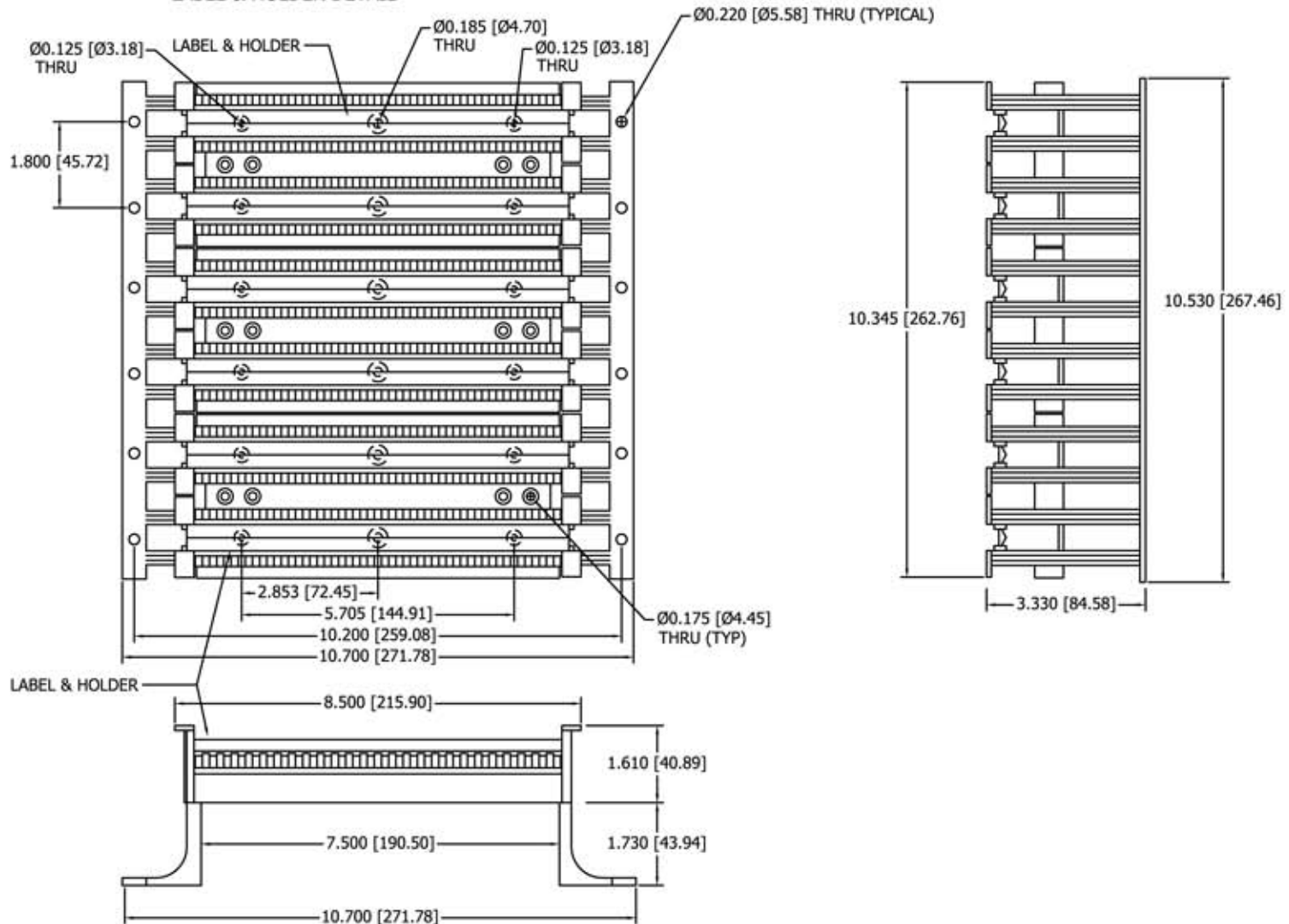
LABEL & HOLDER DETAIL
