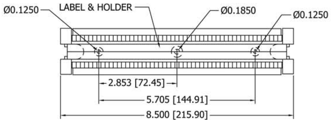
LABEL & HOLDER DETAIL
