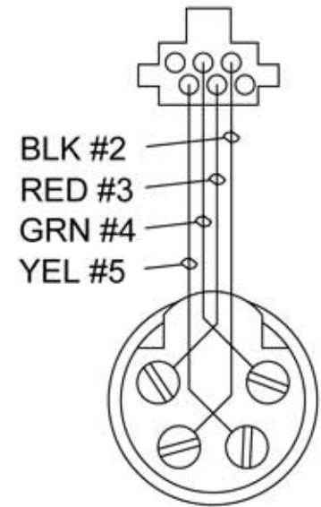
WIRE CONNECTIONS REAR VIEW
