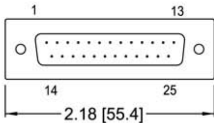
ATRA8M-MALE
