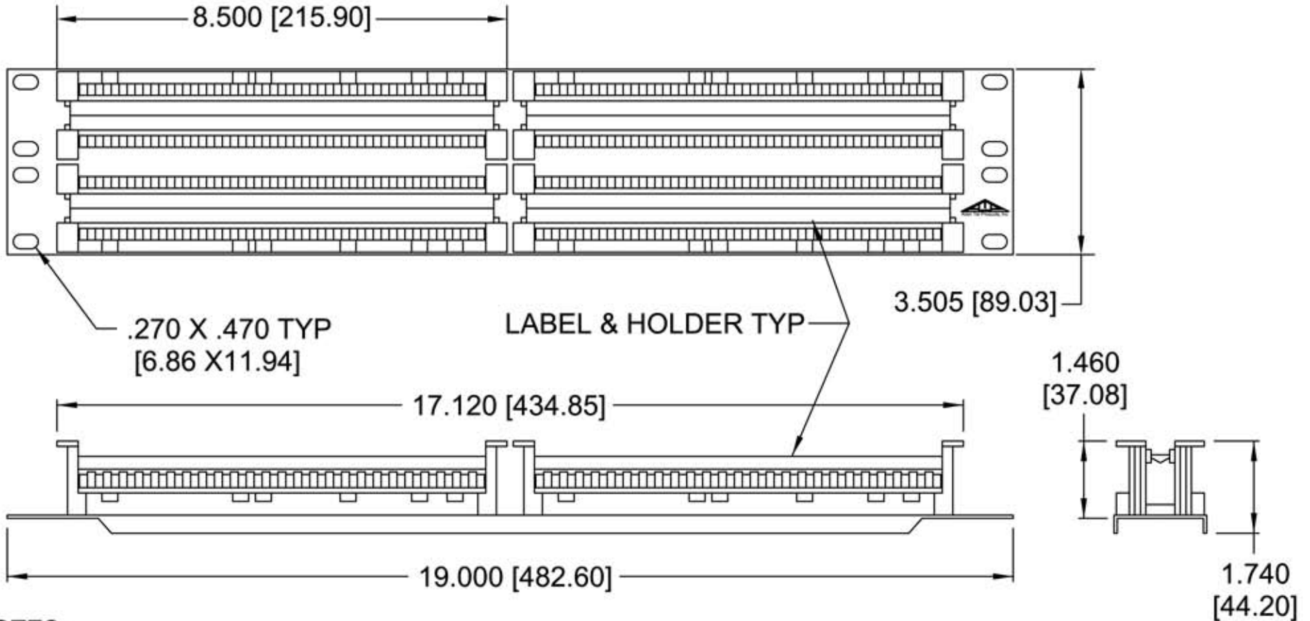
LABEL & HOLDER DETAIL
